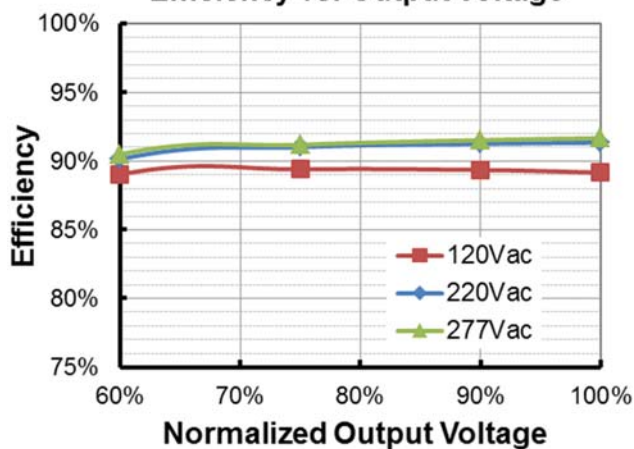
EUM-150S420Dx(I o =2800mA) Efficiency vs. Output Voltage
